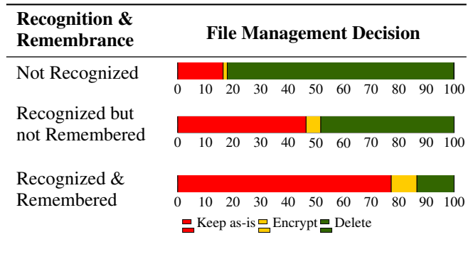
Figure 4: Participants’ management decisions across the possible combinations of file recognition and remembrance. These differences are statistically significant ( \chi^2(4, N = 1000) = 260.26, p < .001 ).
