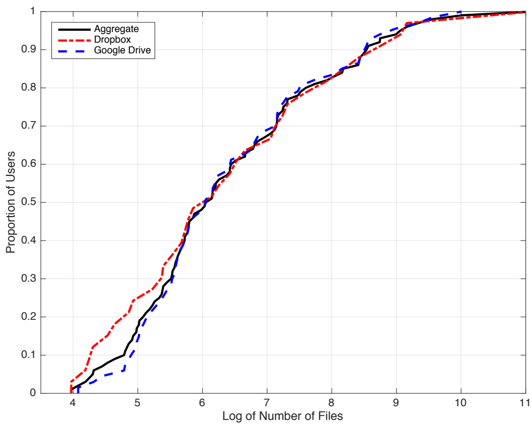
Figure 11: The distribution of (the natural logarithm of) the number of files in participants' accounts. Dropbox and Google Drive follow similar trends.
