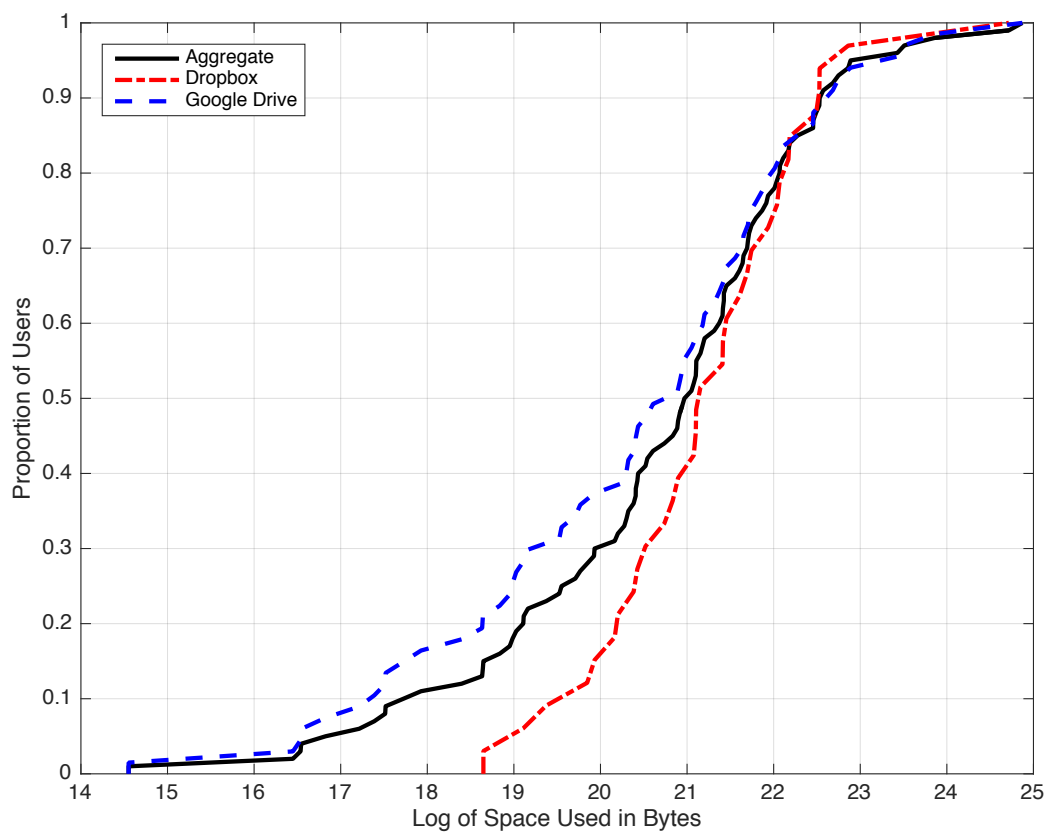
Figure 10: The distribution of how participants' accounts varied in (the natural logarithm of) the number of bytes stored. Dropbox and Google Drive follow similar trends.
