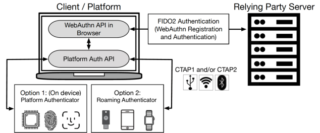
Figure 1: FIDO2 authentication with WebAuthn and CTAP2. This diagram is taken from Lystani et al. [16].
